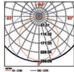
NBTLED T5P14/12 14W
