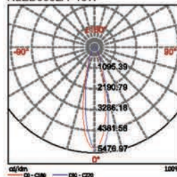
NLED5852A 18W
