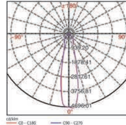
NLED1103D 20W
