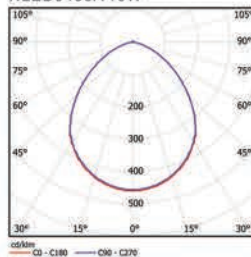
NLED9435A 10W
